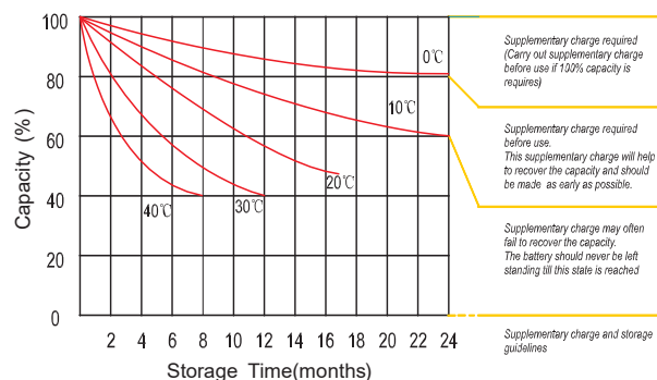
Storage Characteristics
